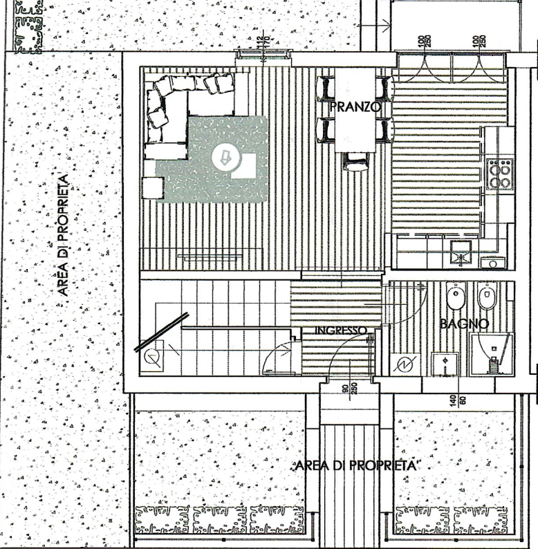
PIANO TERRA
